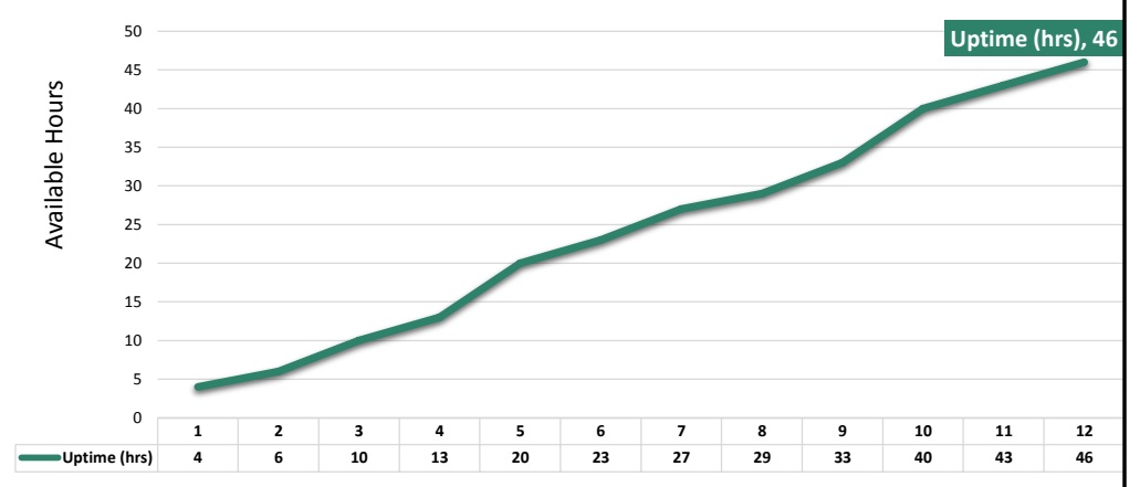
AVAILABILITY INCREASE WITH ZEMEK STRAIGHT LINE SOCKETS
